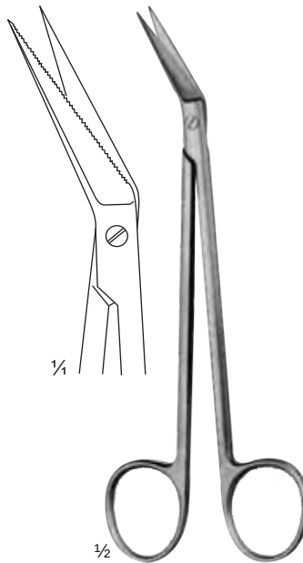
Locklin 06-441-16 16 cm / 6¼" serrated
