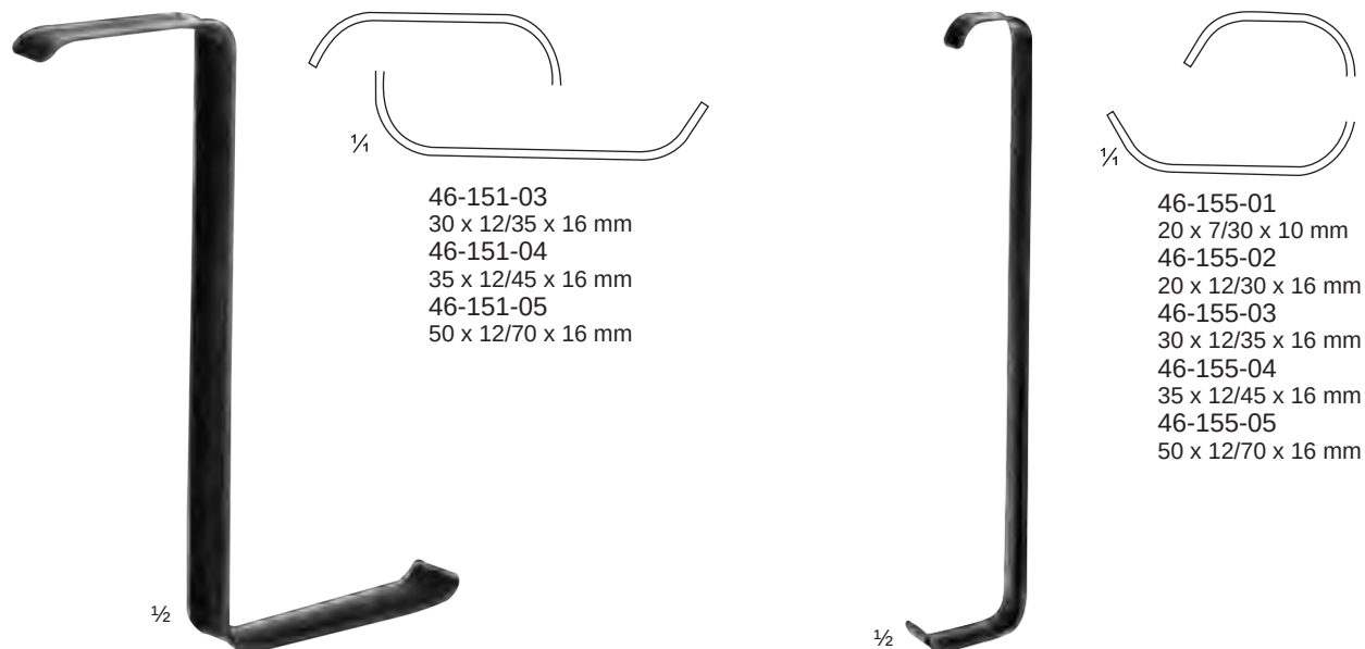
Tessier 46-151-03 - 46-151-05 16 cm / 6 1/4" Black chromium-plated
